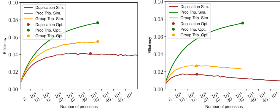
Figure 3: Impact of the number of processes on the efficiency with MTBE = 10^4 (left), MTBE = 10^3 (right), and c = 1800 , d = 0 , \alpha = 10^{-5} .
