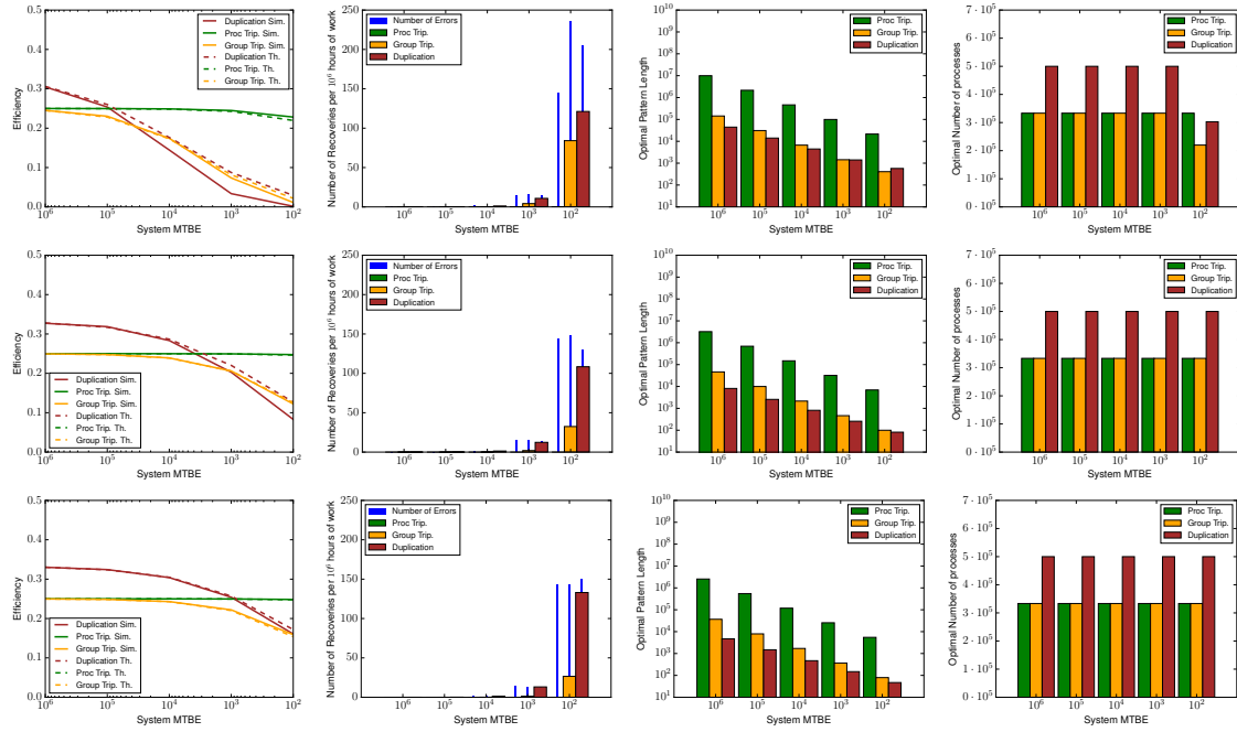
Figure 1: Impact of the system MTBE on the efficiency with c = 1800, d = 0 (top), c = 60, d = 0 (middle), c = 0, d = 10^7 (bottom) and \alpha = 10^{-6} .
