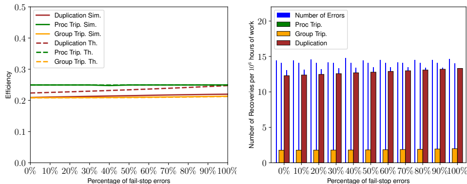
Figure 4: Impact of fail-stop errors as a percentage of the total number of errors with combined MTBE = 10^3 , c = 60 , d = 0 , and \alpha = 10^{-6} .
