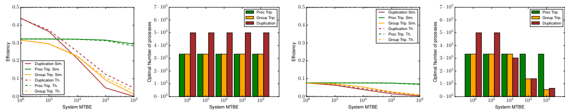
Figure 2: Impact of the sequential fraction (in Amdahl's Law) on the efficiency and optimal number of processes with \alpha = 10^{-7} (left) and \alpha = 10^{-5} (right).
