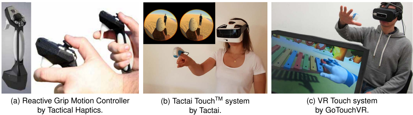
Fig. 6. Gaming is one of the most promising application for wearable haptic technologies. For example, (a) the “Reactive Grip” motion controller provides skin stretch and relative tangential motion to the hand to recreate the compelling sensation of holding in-game objects; (b) the “Tactai Touch™” fingertip device is able to provide pressure, texture, and the sensation of making and breaking contact with virtual objects; and (c) the “VR Touch” fingertip device is able to provide pressure and the sensation of making and breaking contact with virtual objects.
