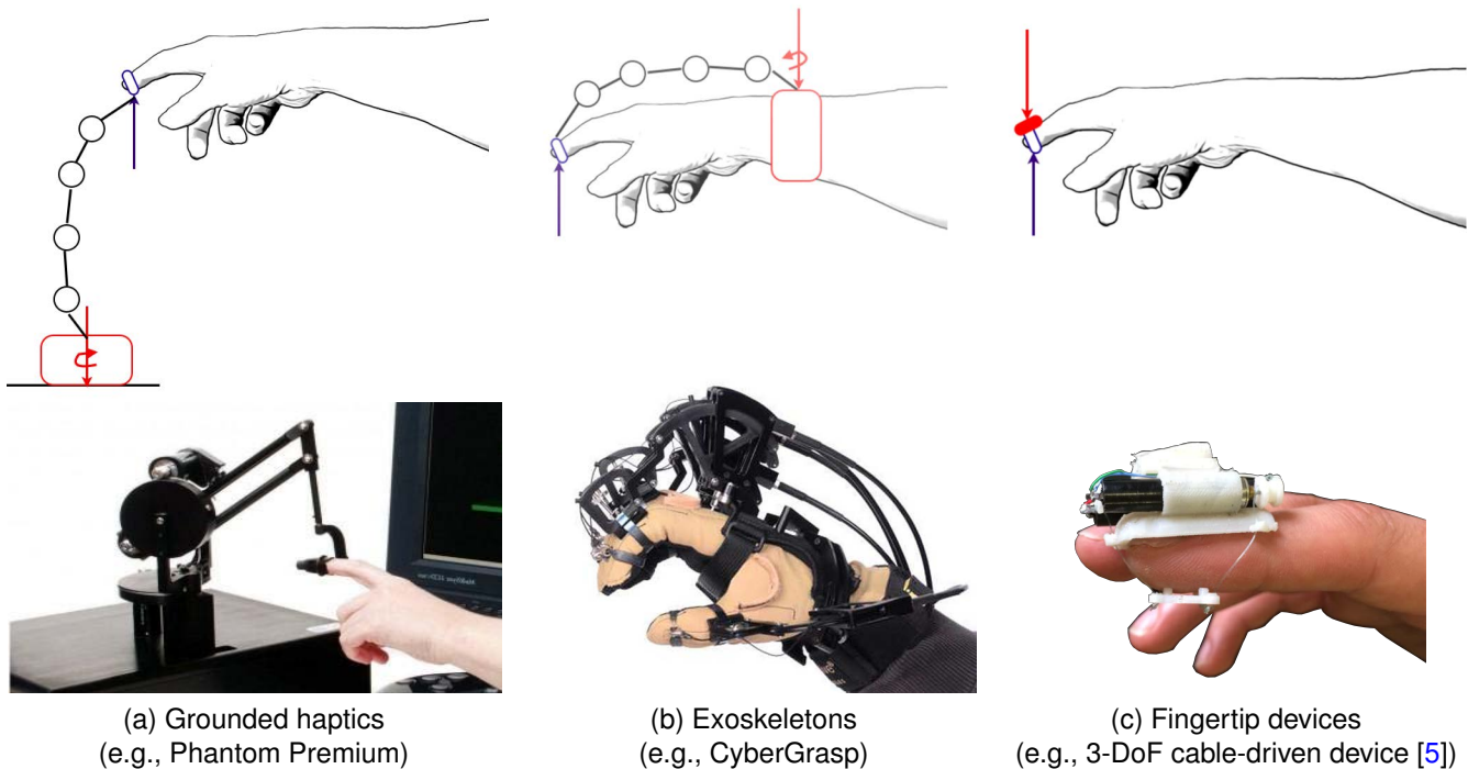
Fig. 1. From grounded haptics to more wearable and portable designs. A Phantom Premium (a), a CyberGrasp (b), and (c) a fingertip device [5]. As we move from (a) to (c), the wearability of the system is improved at the cost of losing part of the kinesthetic component of the interaction.
