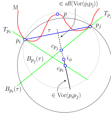
Figure 8.4: The figure shows an example of an inconsistent simplex \sigma = [p_i, p_j] that belongs to \text{star}(p_i) and does not belong to \text{star}(p_j) . The bisector of \sigma is subdivided in two line segments: the solid black line segment belongs to \text{Vor}(\sigma) and the dashed black line segment belongs to \text{aff}(\text{Vor}(\sigma)) but not to \text{Vor}(\sigma) .
