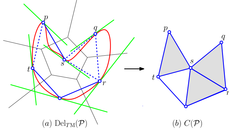
Figure 8.5: Figure (a) shows \mathcal{M} , the sample P , the tangent lines at the sample points, the Voronoi diagram of P and \text{Del}_{TM}(P) . The dashed lines indicate the inconsistent edges. In Figure (b), the line segments denote \text{Del}_{TM}(P) and the grey triangles denote the inconsistency triggers.
