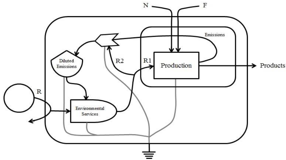
Fig. 1. - To drive production (poultry or aquaculture), flows of renewable ( R_1 ), nonrenewable ( N ) and purchased resources ( F ) are needed (represented by - ) Emissions are diluted by nature through renewable services ( R_2 ). Flows of energy dispersion is represented by -
