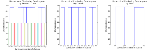
Fig. 2: Hierarchical clustering dendrograms
