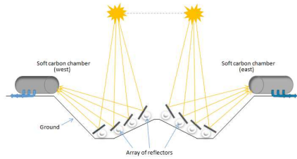
Fig. 2. Implementation scheme of the reflector device
