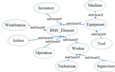
Fig. 3. RMS Ontology
