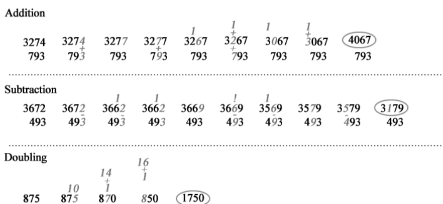
Fig. 1. Examples of Addition, Subtraction, and Doubling
