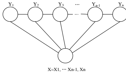
Fig.1. CRFs Model
