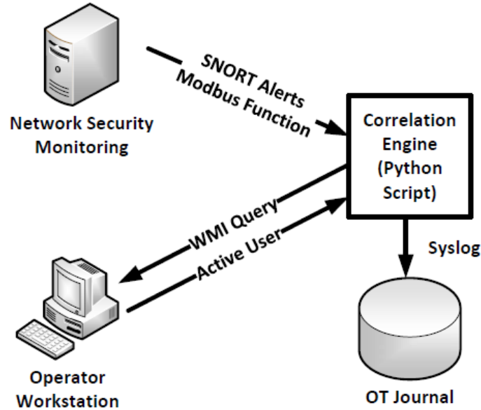
Figure 4. Proof-of-concept implementation.
