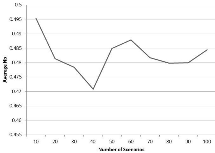
Figure 6. SIM2 N avg values for 100 executions of 10 to 100 scenarios.
