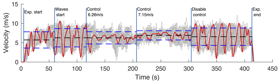
(b) Velocity profiles of all vehicles (gray) and the CAT Vehicle (red) in Experiment B. Horizontal blue dashed lines are one standard deviation above and below the mean speed of traffic in the interval.
