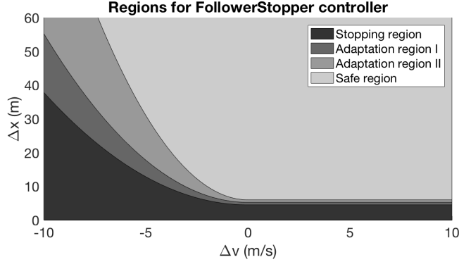
Figure 2: Regions defined in FollowerStopper controller.
