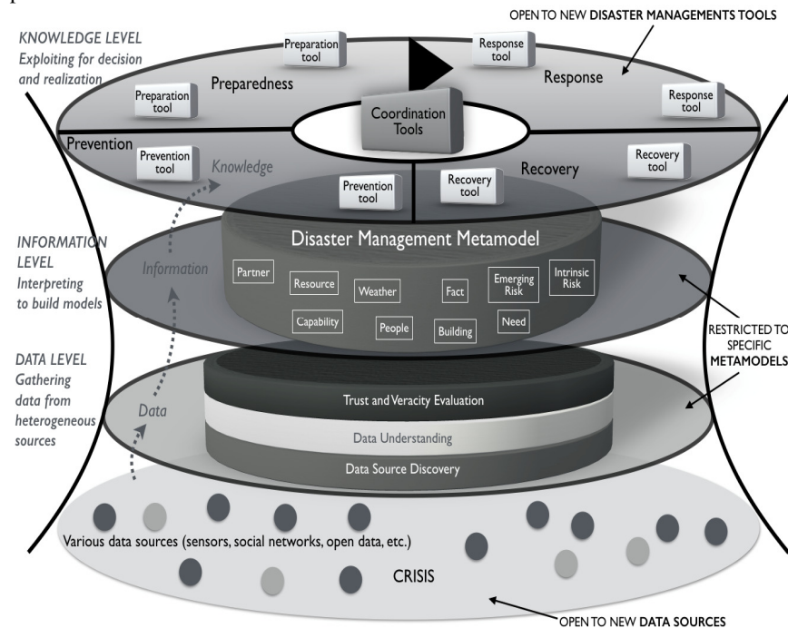
Fig. 1. Big Picture of the Big-Data for DM framework.
