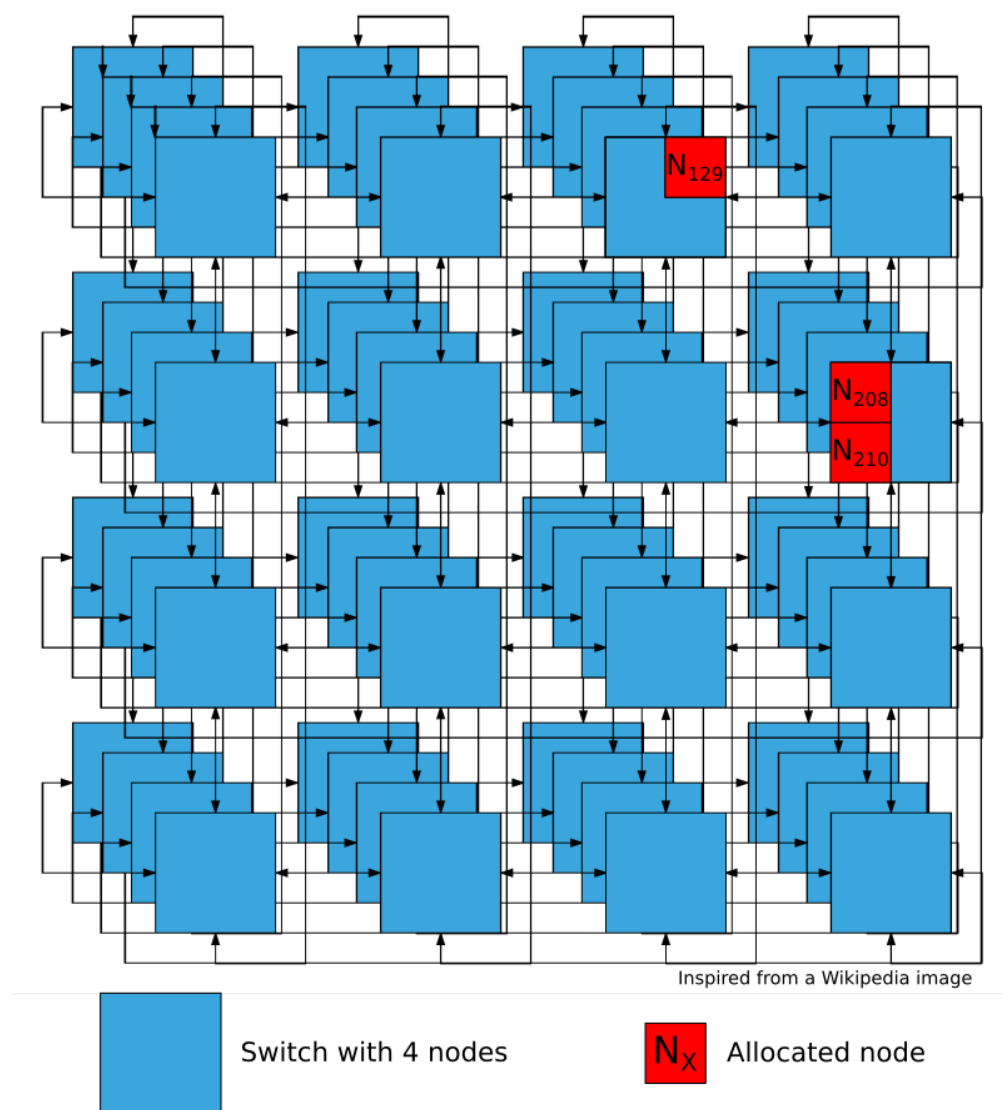
Figure 5: Example of a 3d torus machine with 3 allocated nodes.
