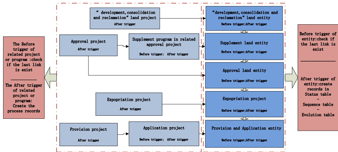
Figure 7. The synchronized updating mechanism of spatio-temporal data based on trigger
