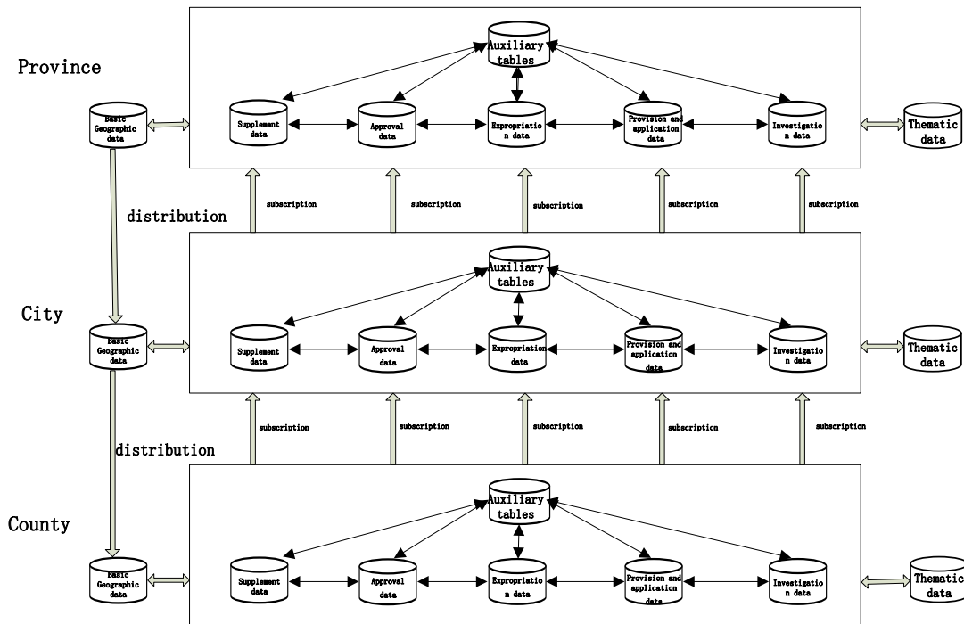
Figure 5 New data flow of construction land supervision database system in distributed environment
