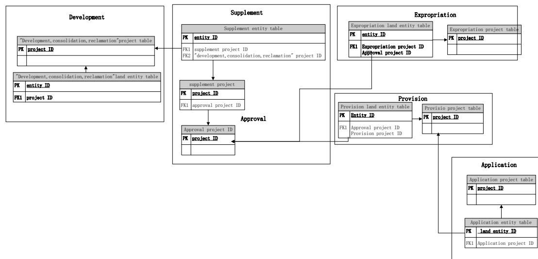
Figure 1 storage structure of the basic table data in supervision database
