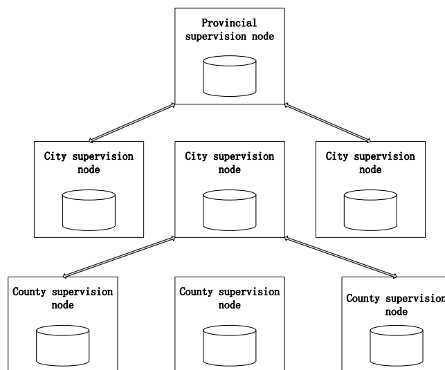
Figure 4. Construction land use supervision database management system in “province-city-county” three-level network environment
