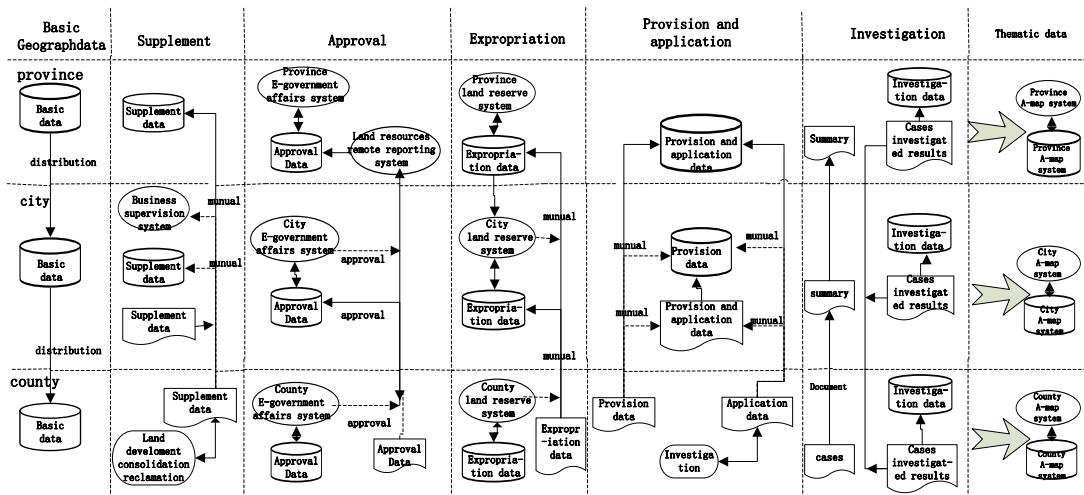
Figure 3. The supervision data flow status in “province-city-county” distributed environment
