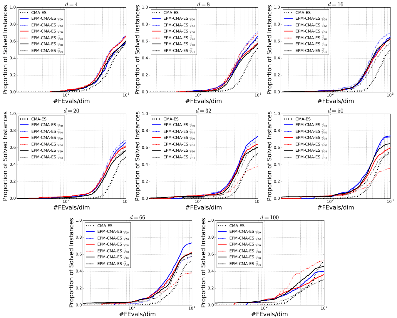
Figure 3: ECDF comparing EPM-CMA-ES with \psi_k or \widehat{\psi}_k ( k \in \{10, 30, 50\} ), and default CMA-ES.
