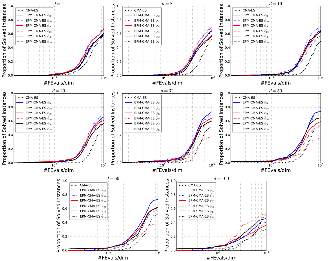
Figure 3: ECDF comparing EPM-CMA-ES with \psi_k or \widehat{\psi}_k ( k \in \{10, 30, 50\} ), and default CMA-ES.
