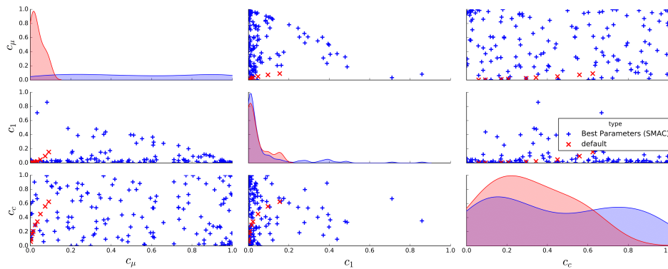
Figure 2: Comparison of the default (×) and best (+) parameter setting for c_1 , c_\mu and c_c parameters of CMA-ES, for each function from BBOB and each dimension d \in \{2, 4, 5, 8, 10, 16, 20, 32, 40, 64\} . Two axes projections are displayed out-diagonal, while density distributions for the corresponding parameter are shown on the diagonal.
