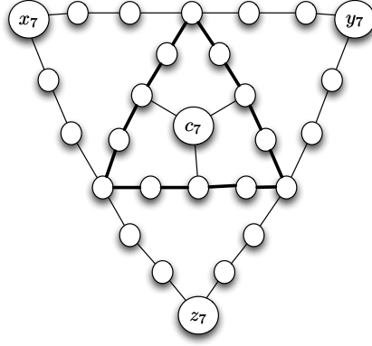
FIGURE 2. Example of T_7 . Edges are bold only to better distinguish the different “levels”.
