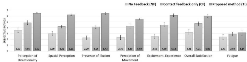
Fig. 2. Responses to the UX questionnaire for and differences among the three feedback methods (the error bars indicate the standard error of the mean).
