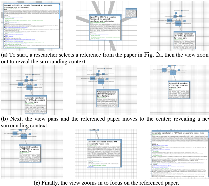
Fig. 4. Focus-Context-Focus Hop
