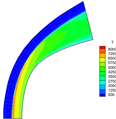
Figure 13: Simulation of the hypersonic flow around the nose of EXPERT vehicle, performed with COSMIC code: temperature field at nominal freestream conditions at 60km altitude.
