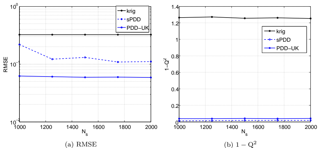
Figure 5: TEST 4: Actual (RMSE) and cross-validation ( 1 - Q^2 ) error measures when increasing the number of training points. Results are plotted for the Ordinary Kriging, Sparse-PDD and coupled PDD-UK surrogate models of the 100-dimensional Sobol function. Variance-based adaptive algorithm.
