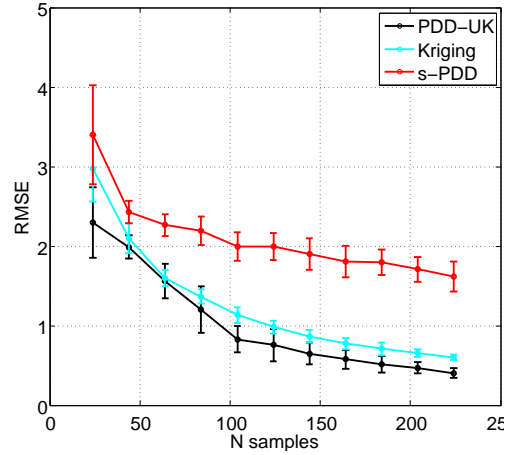
Figure 3: TEST 1: Mean RMSE convergence comparison between Ordinary Kriging, sparse PDD and coupled PDD-UK metamodelling methods, m = 5
