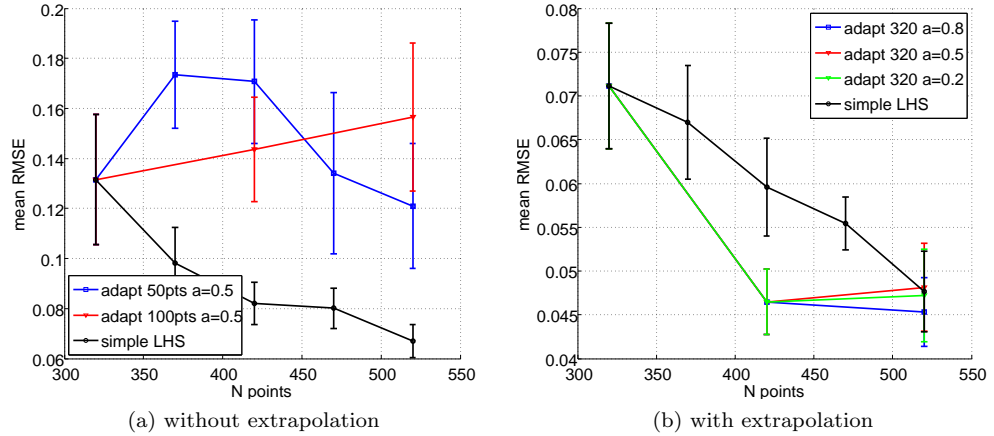
Figure 11: 8D Testcase: Convergence of the mean value of the RMSE and corresponding deviation computed with 14 different starting LHS DoE. The result of a simple increase of LHS point is compared with adaptation at different values of \alpha coefficient. A comparison is done between the normal algorithm and the one with extrapolation near the corners of the domain
