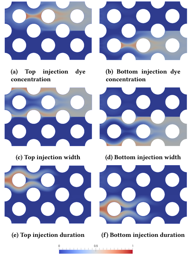
Figure 7: First order Sobol' index maps on a slice of the mesh at timestep 80. The left column corresponds to the Sobol' indices for the upper injector while right corresponds to the bottom injector. All maps are scaled between zero (blue) and one (red).
