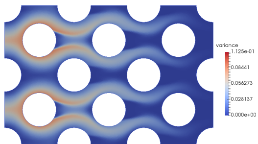
Figure 8: Variance map at the 80 th timestep
