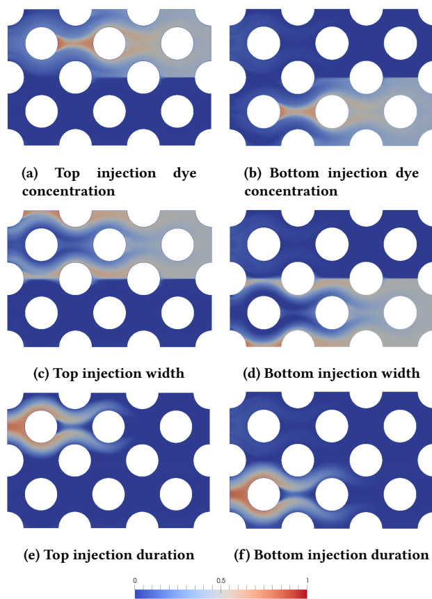
Figure 7: First order Sobol' index maps on a slice of the mesh at timestep 80. The left column corresponds to the Sobol' indices for the upper injector while right corresponds to the bottom injector. All maps are scaled between zero (blue) and one (red).
