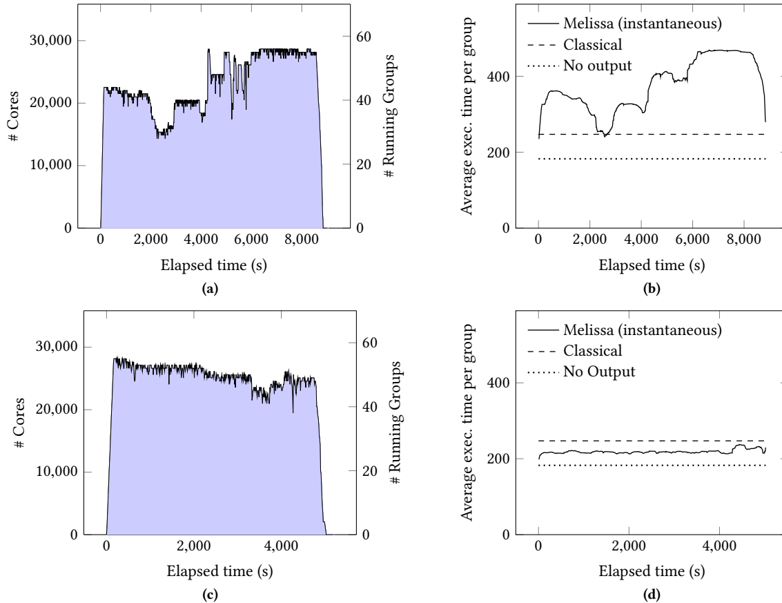
Figure 6: Two sensitivity analysis en Curie. The first one ran Melissa Server on 15 nodes (top plots (a) and (b)), the second ran with Melissa Server on 32 nodes (bottom plots (c) and (d)). Left: evolution of the number of running simulation groups (and number of cores used) during the experiment. Right: average execution time of the running simulation groups during the experiment.
