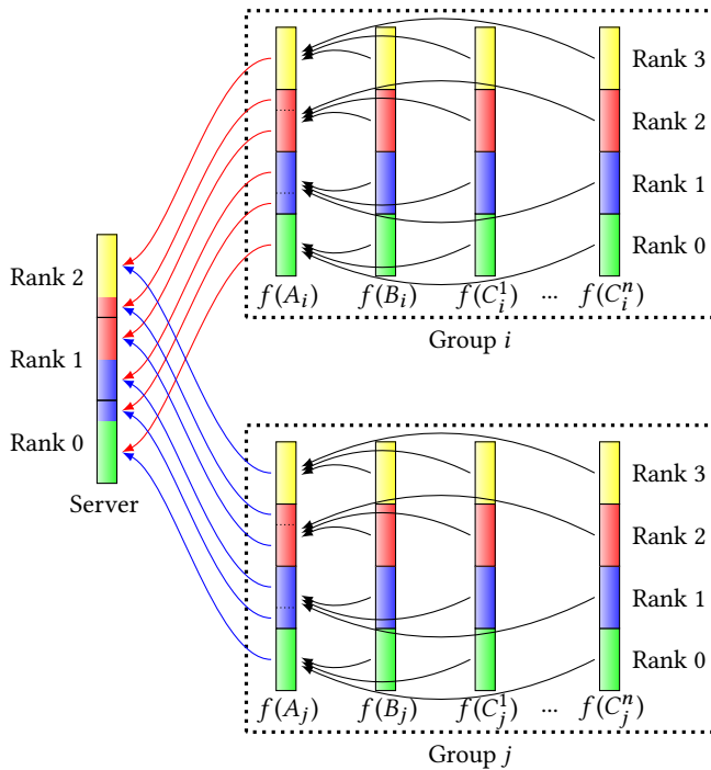
Figure 4: Two simulation groups i and j , each running n + 2 parallel simulations (4 processes), are connected to the Melissa parallel server (3 processes). Each time the results of a new timestep are available within a group, the data are first gathered on the main simulation processes (black arrows), before to be redistributed to the server (blue and red arrows).
