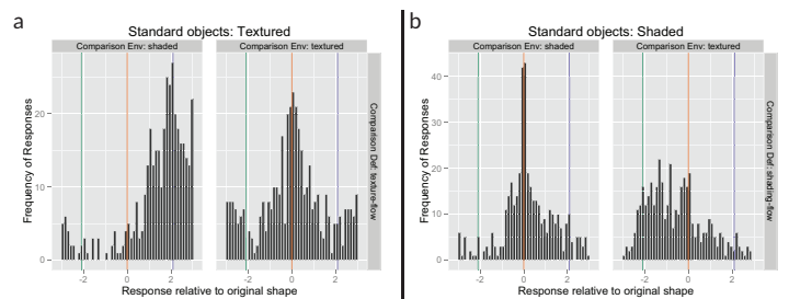
Figure 3: Observers judgments for textured (a) and shaded (b) standard objects. Judgments are relative to the true shape (Fig. 1a) at 0 (orange marker). The shape from Fig. 1b is at -2\pi/3 (green marker), while the object from Fig. 1c is at 2\pi/3 (blue marker). Note the effect of surface appearance, with matches near the base shape when the standard’s cue and comparison’s environment match.
