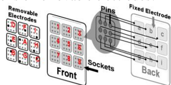
Fig 4. Design of a reconfigurable CipherCard.
