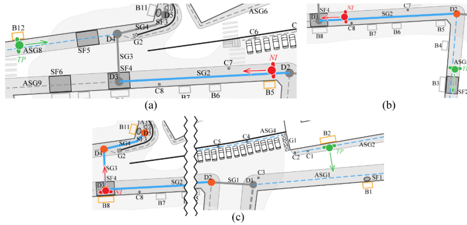
Fig. 3. Similarities in sessions S 5 (a), S 11 (b), and S 18 (c). The green figure represents the traveler's physical position and direction (TP). The red figure represents the navigator's imagination of the traveler's physical position and direction (NI).
