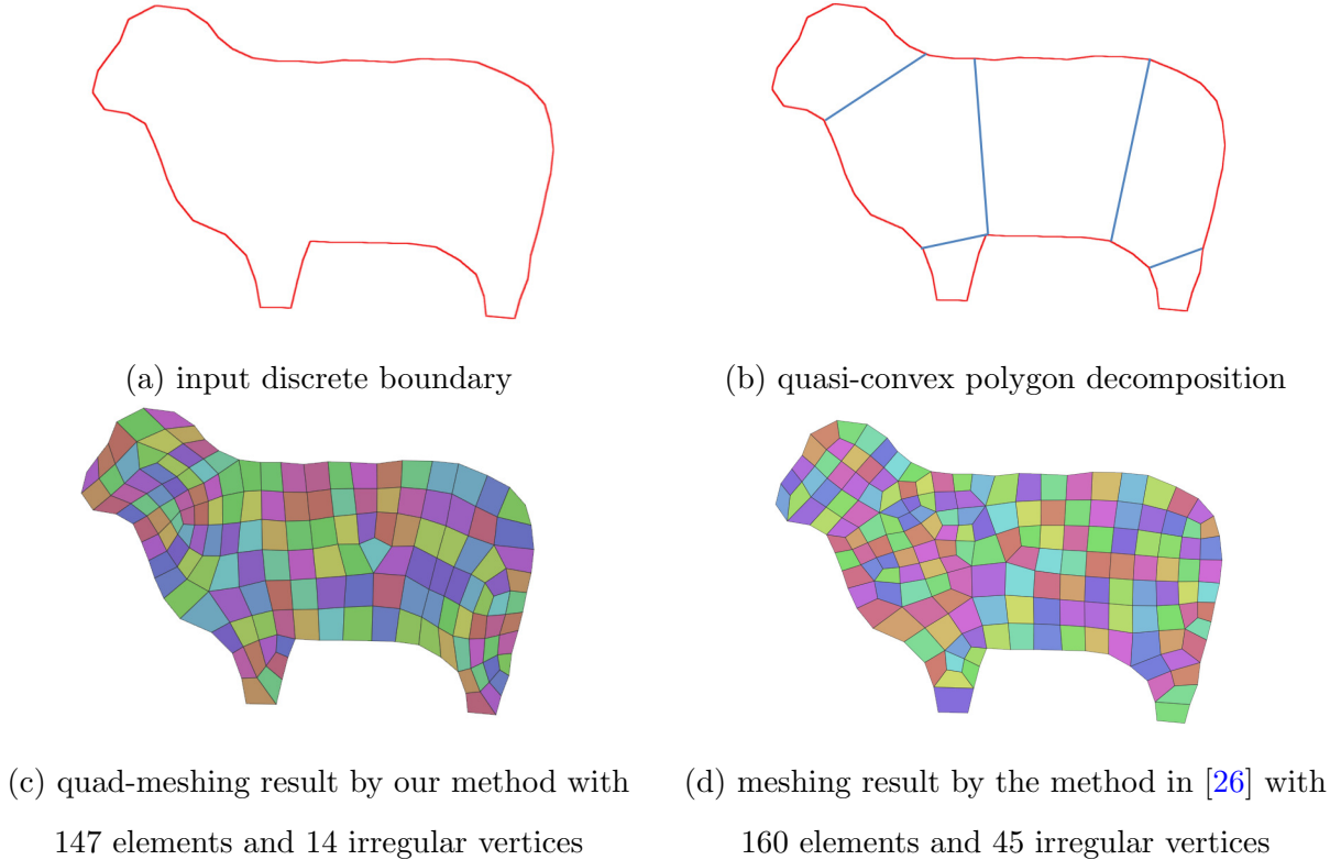
Fig. 3. Quad-meshing example.
