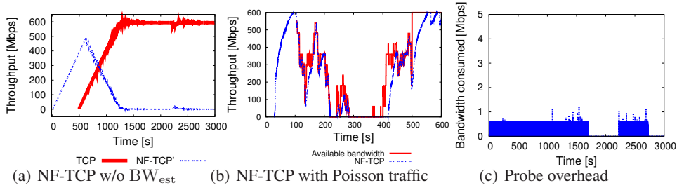
Fig. 7. Need for bandwidth estimation and the low overhead it produces
