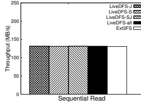
Fig. 8. Throughput of sequential read.
