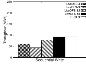
Fig. 7. Throughput of sequential write.
