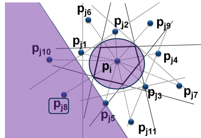
Figure 3: The Voronoi cell V(p_i) is the intersection of the halfspaces defined by the bisectors of the segments [p_i, p_j] . Once a point (here p_{j_8} ) is further away twice than the current Voronoi cell at p_i , it no longer contributes to the cell.
