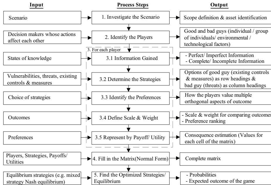
Fig. 2. Input and Output for Game Theoretical Steps
