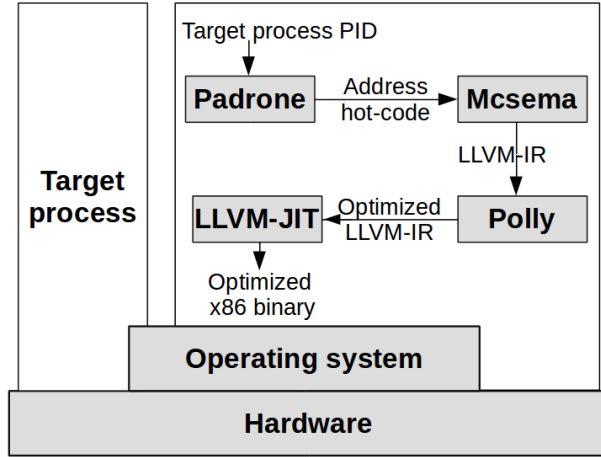
Fig. 11 Auto-vectorization process
