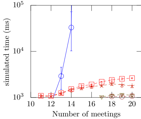
(c) Time complexity
