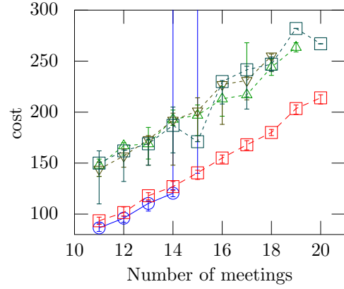
(b) Comparison with alternatives
