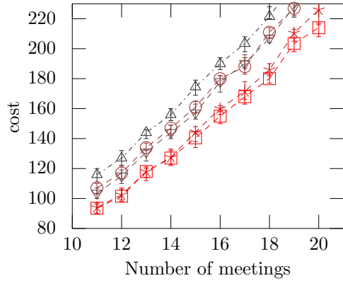
(a) Comparison between DUCT variants
