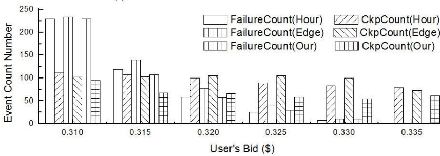
Fig. 15. Performance comparison of checkpointing schemes in m1.xlarge
