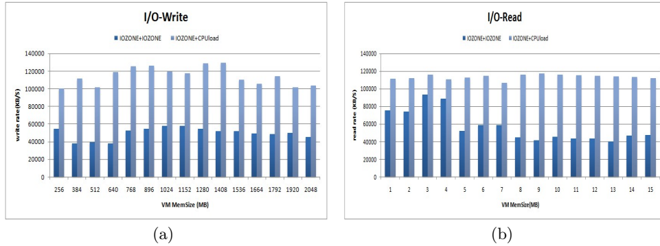
Fig. 3. Two I/O type VMs working together
