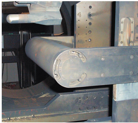
Figure 2: Image of the cylindrical experimental model in the HEG facility (taken from [11]).
