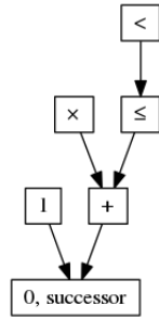
Fig. 1. The FoCaLiZe species hierarchy of MathTransfer structures
