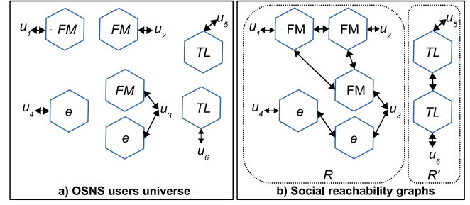
Fig. 1. Social reachability graph
