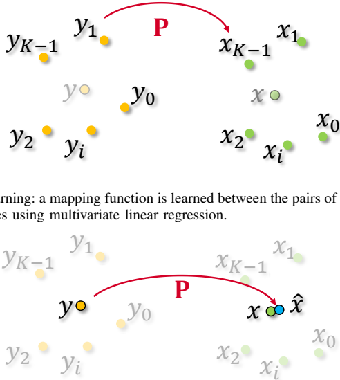
Fig. 8. Two steps local learning-based restoration based on linear regression.
