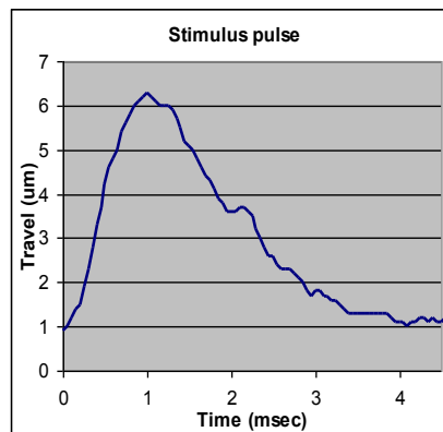
Fig. 3. The tactile feedback pulse used in Experiment 1. The figure shows the displacement of the display module.
