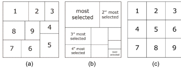
Fig. 5. Abstraction of the three layout options for application zones in SCOTZ: (a) spiral treemap, where applications are (arbitrarily) sorted once and this ordering is retained forever, and where zones are laid out in order in a clockwise spiral from top left; (b) squarified treemap, where application zones are sorted by size and laid out from top left to bottom right; (c) grid, where all application zones are of equal size and are laid out in a grid pattern.
