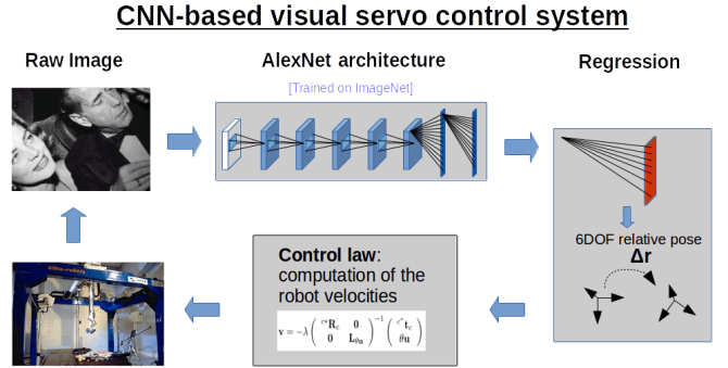
Figure 1. Overview of the proposed CNN-based visual servo control system
