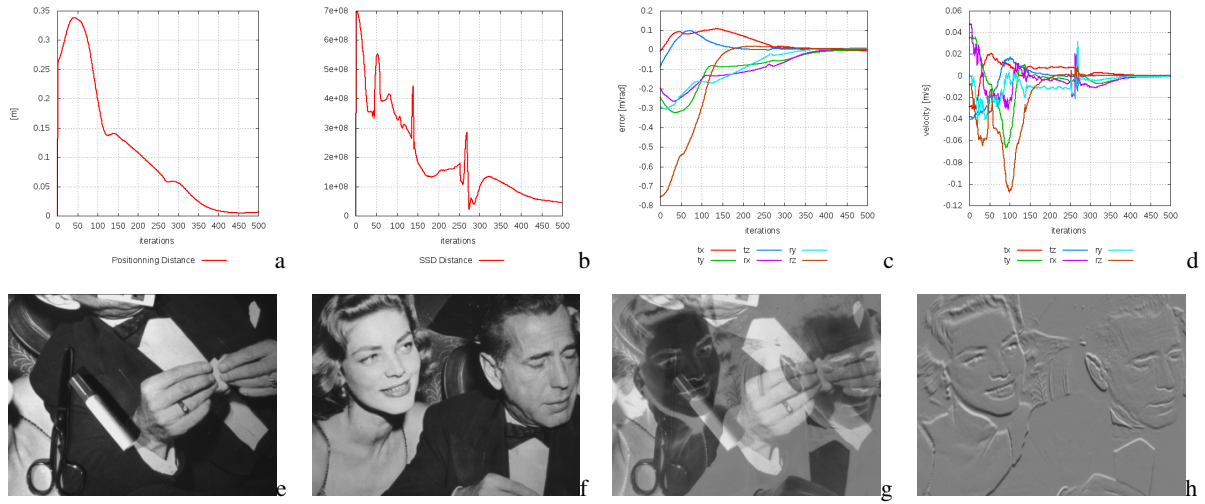
Figure 6. CNN-based visual servoing on a planar scene with various perturbations. (a) Positioning error; (b) SSD distance; (c) Translational and rotational errors; (d) Camera velocities in m/s and rad/s; (e) Image at initial pose I_0 ; (f) Image at final pose I(\hat{F}) ; (g) Image error I_0 - I^* at initial pose; (h) Image error I(\hat{F}) - I^* at the final pose
