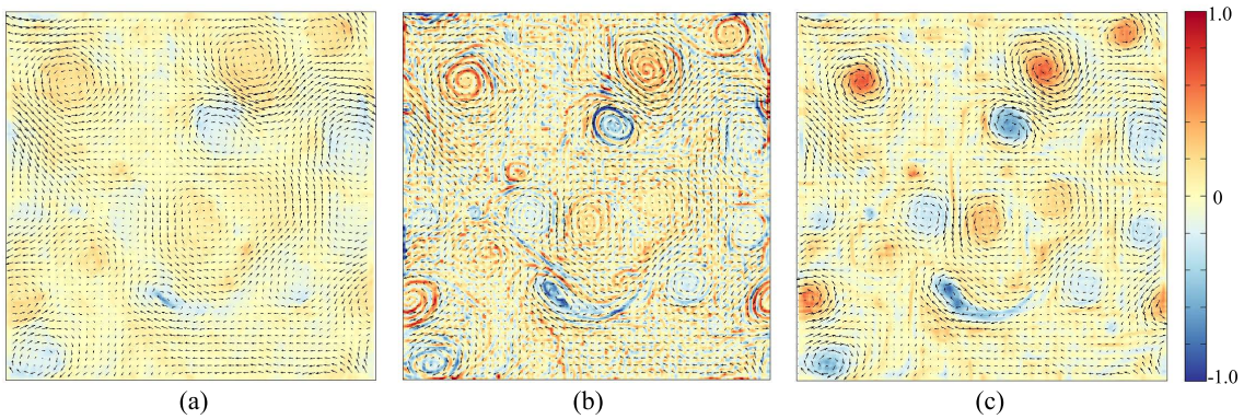
Fig. 10 Results at t = 450 on the synthetic SQG scalar image sequence: (a) estimated velocity field and vorticity map from the HS method; (b) estimated velocity field and vorticity map from Dérian et al. (2013); (c) estimated velocity field and vorticity map from the proposed method.
