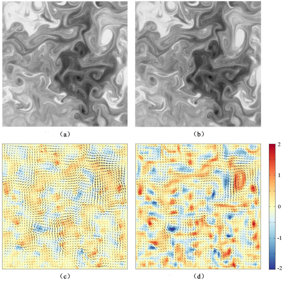
Fig. 12 Results on experimental scalar images: (a) first frame; (b) second frame; (c) estimated velocity field and vorticity map from the HS method; (d) estimated velocity field and vorticity map from the proposed method.
