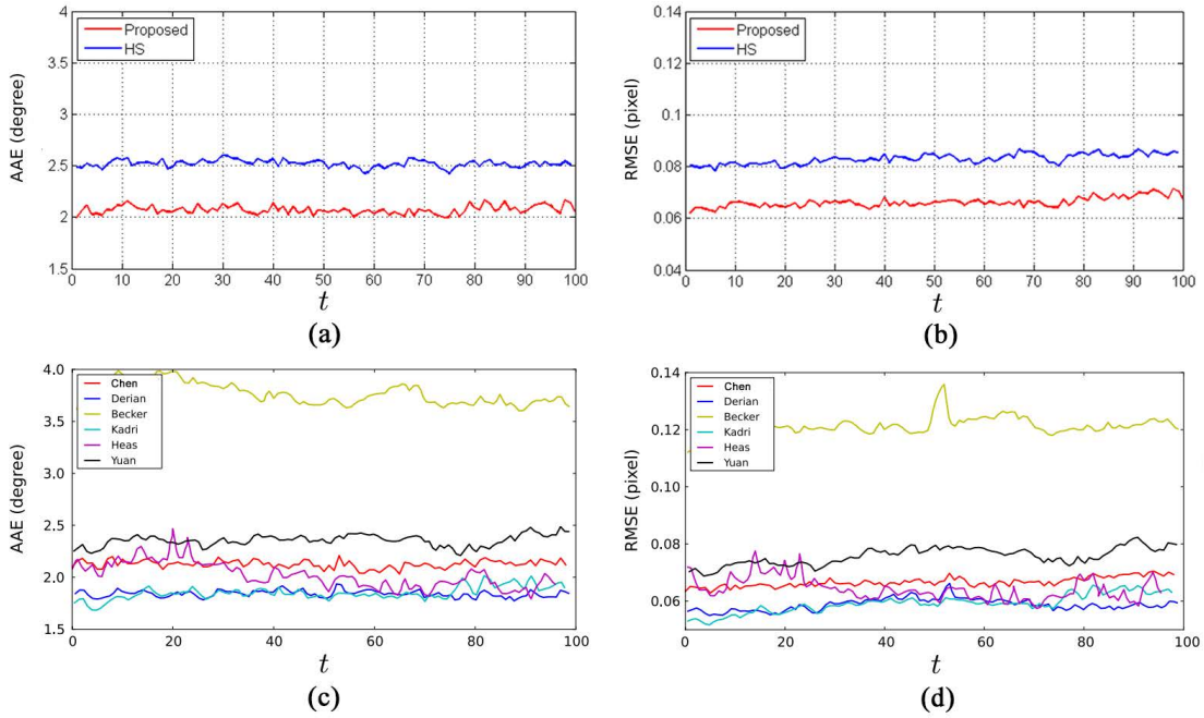
Fig. 6 AAE (left) and RMSE (right) errors of different estimators for DNS particle image sequence. Results of the proposed method are plotted in figures (a) and (b), in comparison with the results of the HS method. The data of several state-of-the-art approaches, shown in figures (c) and (d), are extracted from Chen et al. (2015).
