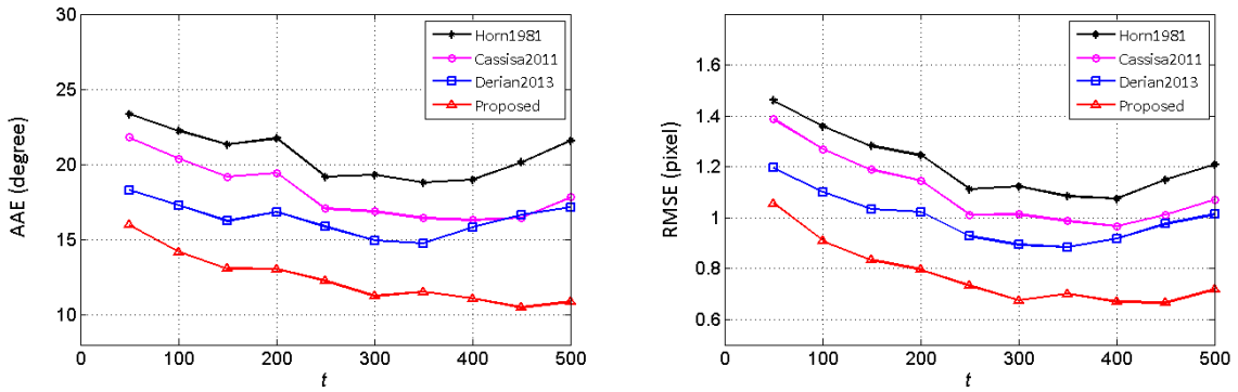
Fig. 9 AAE (left) and RMSE (right) errors for SQG scalar image sequence.
