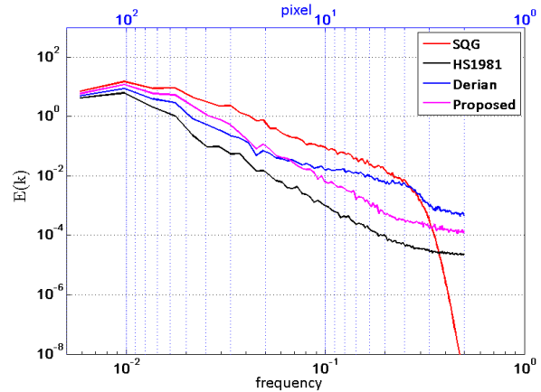
Fig. 11 Spectrum analysis of the turbulent velocity for SQG scalar image sequence.
