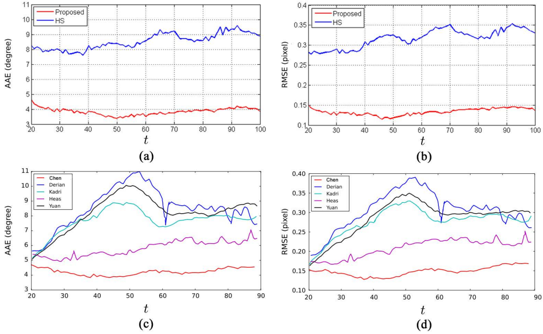
Fig. 4 AAE (left) and RMSE (right) errors of different estimators for DNS scalar image sequence. Results of the proposed method are plotted in figures (a) and (b), in comparison with the results of the HS method. The data of several state-of-the-art approaches, shown in figures (c) and (d), are extracted from Chen et al. (2015).
