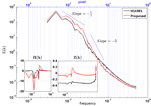
Fig. 13 Spectrum analysis of the turbulent velocity for experimental scalar images. E(k) denotes the energy at a given frequency, \Pi(k) and Z(k) the energy flux and entrophy flux, respectively.
