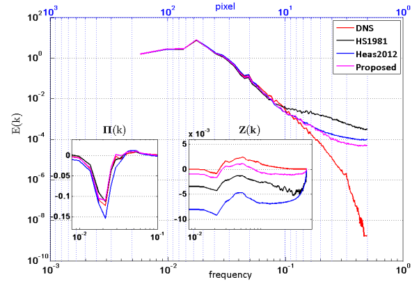
Fig. 7 Spectrum analysis of the turbulent velocity for DNS particle image sequence. E(k) denotes the energy at a given frequency, \Pi(k) and Z(k) the energy flux and enstrophy flux, respectively.
