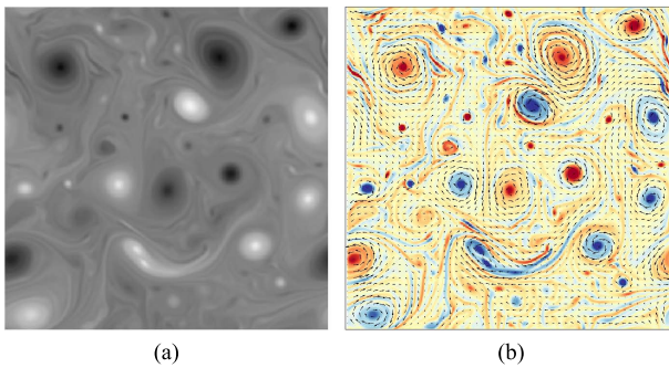
Fig. 8 Illustration of a sample frame ( t = 450 ) from the synthetic SQG sequence: (a) passive scalar image; (b) the simulated ground-truth velocity field with vorticity map, which is used for evaluation of the estimated motion hereafter.
