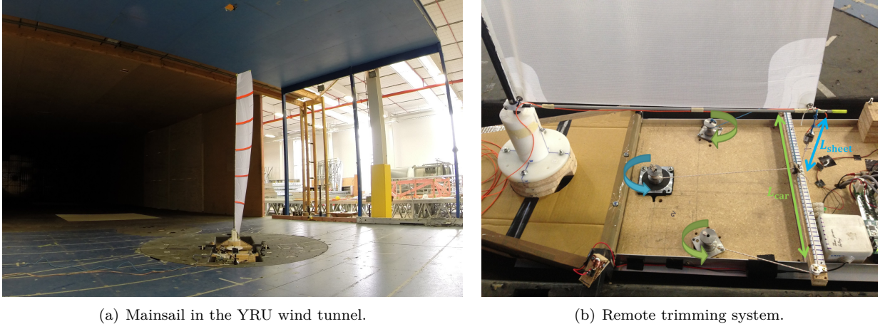
Figure 3: Experimental setup.
