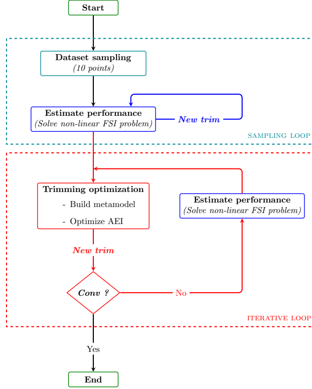
Figure 2: Schematic of the GP-model based optimization procedure.
