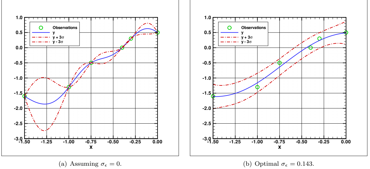
Figure 1: Effect of \sigma_\epsilon on the GP model.
