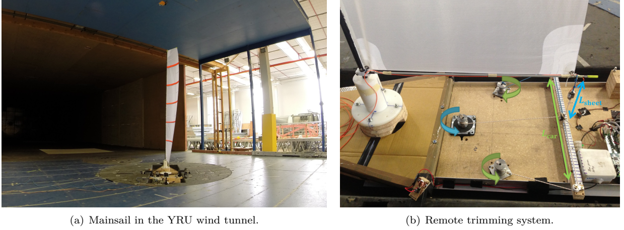
Figure 3: Experimental setup.
