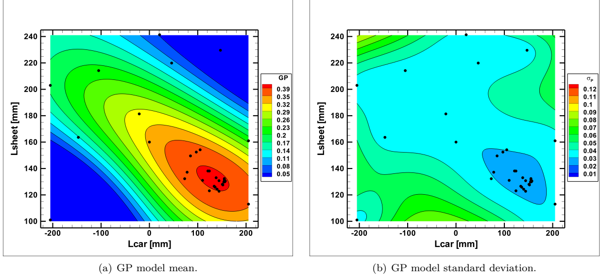
Figure 6: GP model of \mathcal{P}^{\text{exp}}(\mathbf{x}) at iteration 33. Case of \sigma_\epsilon = 0.027 .
