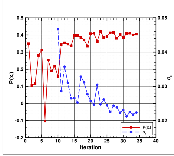
Figure 15: Sequence of computed \mathcal{P}^{\text{num}}(\mathbf{x}_n) as a function of the iteration index (in red, left axis), and corresponding inferred \sigma_e (in blue, right axis). Case of the viscous model.
