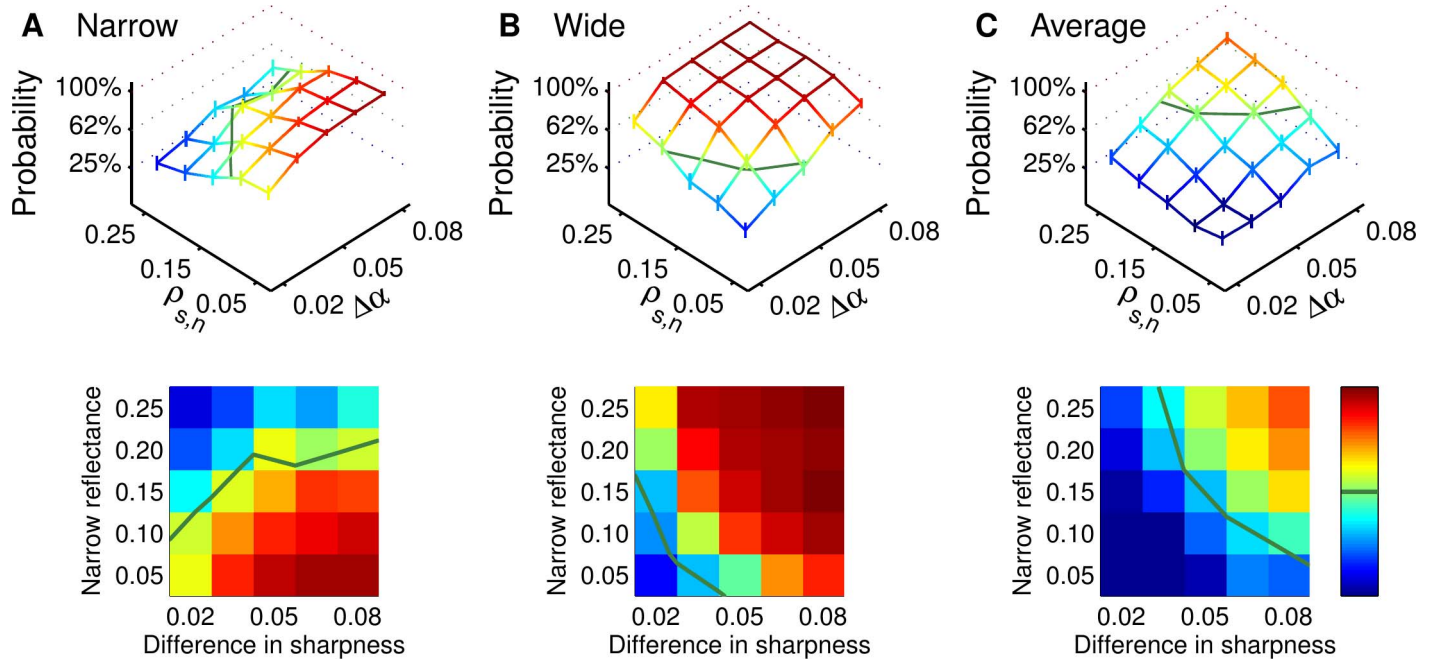
Figure 11. Results of the discrimination task for N = 15 participants for the conditions where the single-component material used the (A) narrow, (B) wide, or (C) average sharpness of the two-component target material. In the top row, the vertices of the color-coded surface indicate mean performance over all participants as a function of the difference in sharpness ( \Delta\alpha ) and the reflectance of the narrow component ( \rho_{s,n} ), with error bars delimiting the 95% confidence interval. The dotted lines indicate chance (25%), threshold (62.5%), and ideal performance (100%). The bottom row is a top-down view of the same results. The dark green line in both rows is the contour of threshold performance.
