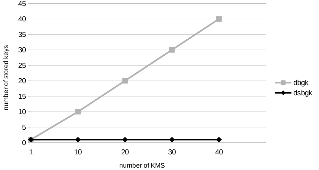
Fig. 3. Storage overhead
