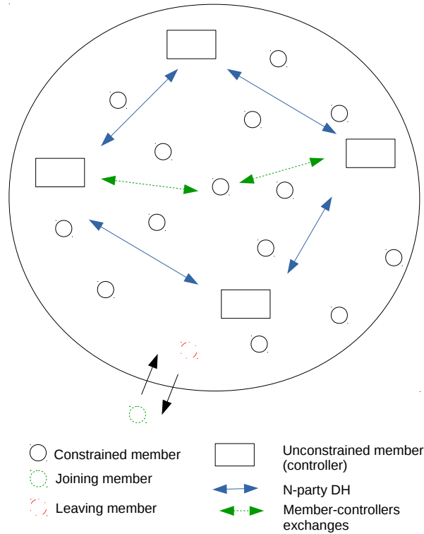
Fig. 2. Network architecture
