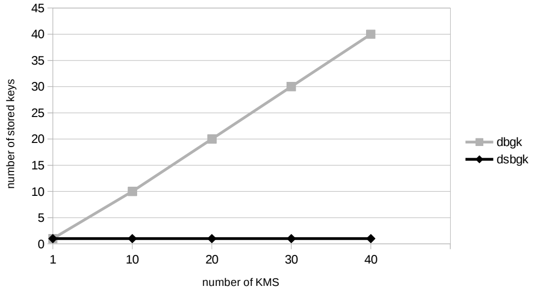
Fig. 3. Storage overhead
