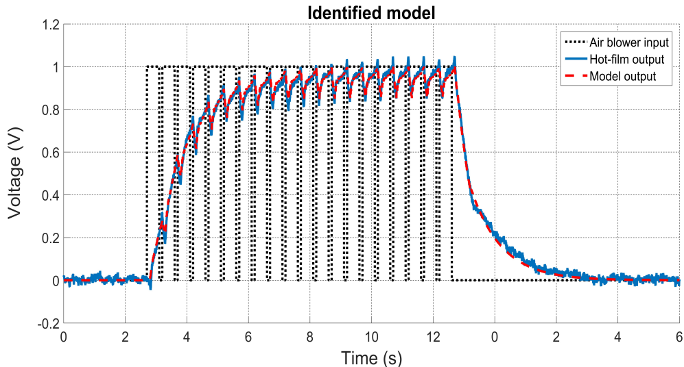
Figure 4: Phase-averaged data for Freq=4Hz, DC=80%
