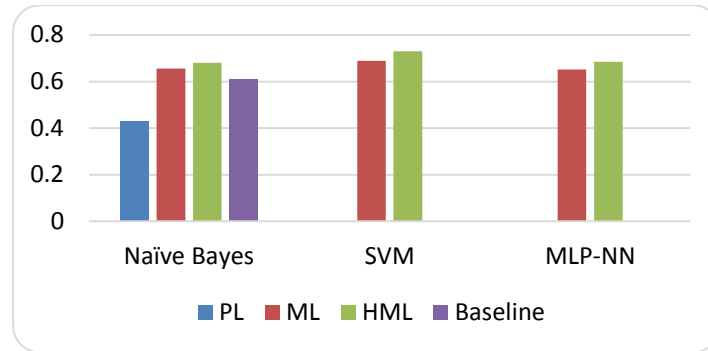
Fig. 3. Evaluation results of the proposed approach - Accuracy
