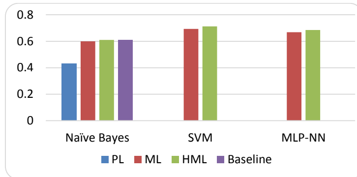
Fig. 4. Evaluation results of the proposed approach - Precision
